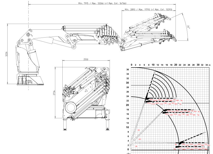
HIAB X-HIPRO 1058 E-8 + JIB 150X-6
