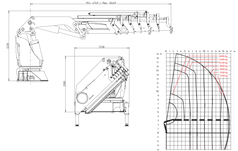
HIAB X-HIPRO 1058 E-8 + JIB 150X-6
